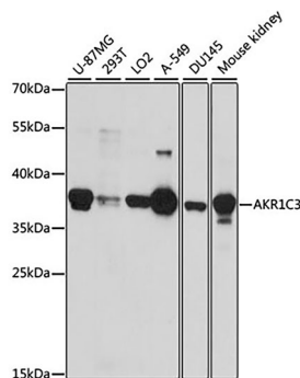
Fig. 1. Western blot analysis of extracts of various cell lines, using AKR1C3 antibody at 1:1000 dilution. Secondary antibody: HRP-labeled Goat Anti-Rabbit IgG(H+L) (A0208) at 1:1000 dilution. Lysates/proteins: 25µg per lane. Blocking buffer: QuickBlock™ Blocking Buffer (P0231). Detection: BeyoECL Star (P0018A). Exposure time: 1s.
